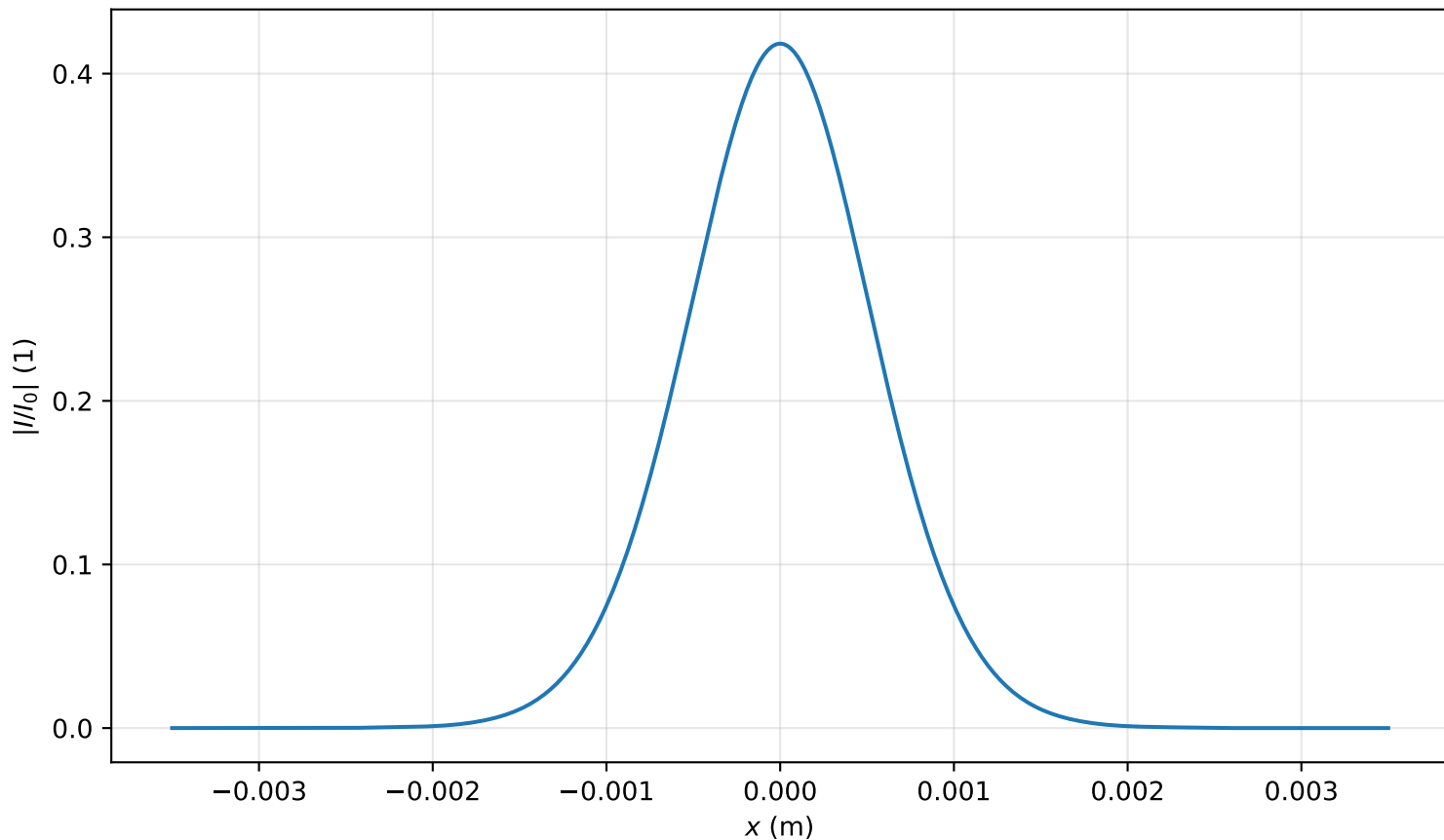
Intensity profile I(x, y = 0, z = 3.025m)/I_0 , P_{in}=0.3P_{cr} , artificial time
